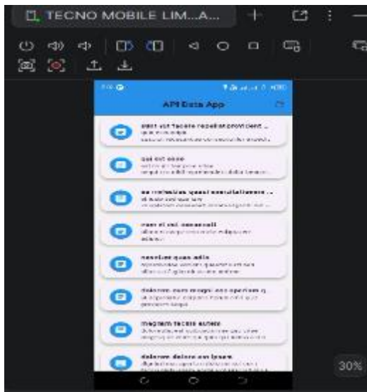
Figure 1: API data
