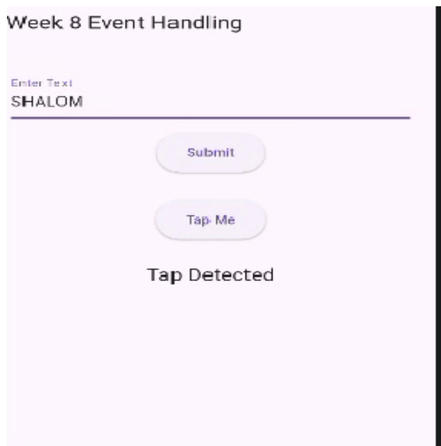
Figure 3: Tap Event
