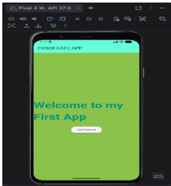
Figure 7:Modified App
