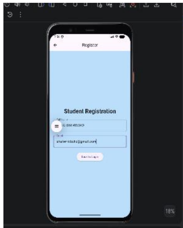
Figure 2:Registration Screen
