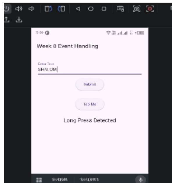
Figure 2: Keyboard input
