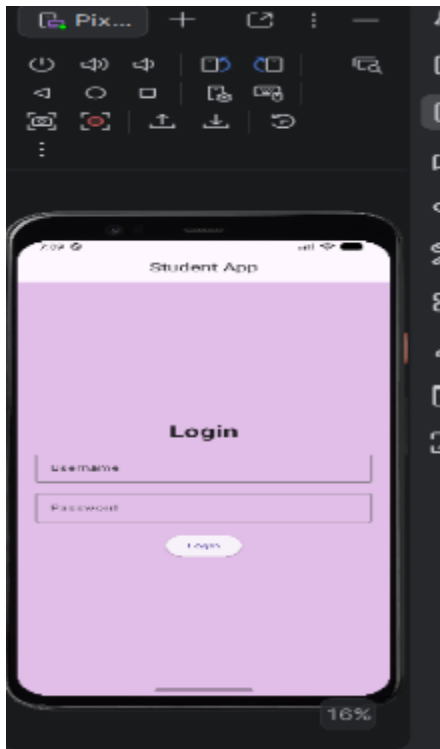
Figure 1:Login Screen
