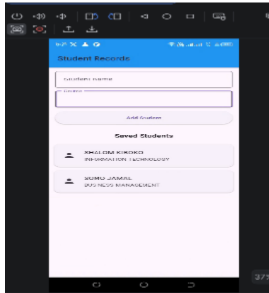
Figure 2: Student Records
