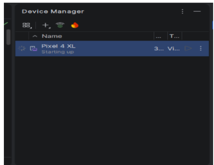
Figure 4: Emulator
