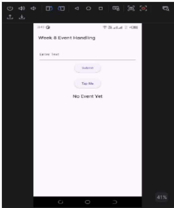
Figure 1: Main Screen
