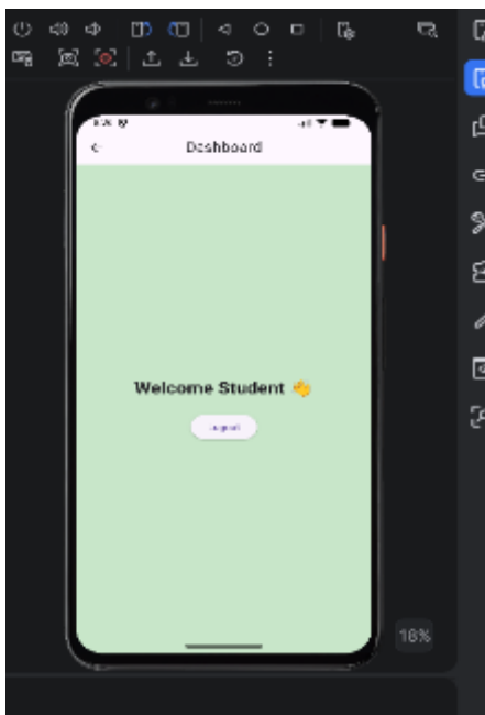
Figure 3: Dashboard Screen
